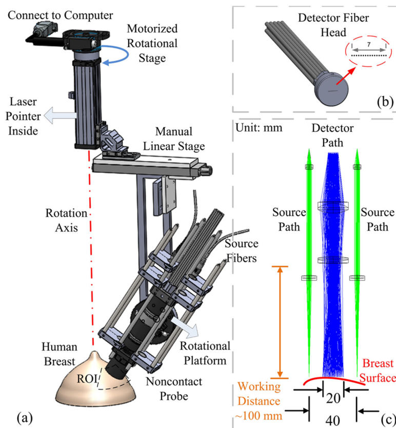
Figure 4. A noncontact DCT probe with rotational scanning system. (a) Noncontact DCT probe head was scanned over a region of interest (ROI) on the breast by a motorized rotational stage, (b) a linear array of single-mode detector fibers, (c) source and detector fibers were projected on the breast surface using achromatic lenses; two source paths were attached to the sides of the detector path. This figure is reproduced from figure 1 in Huang et al (2015b).
