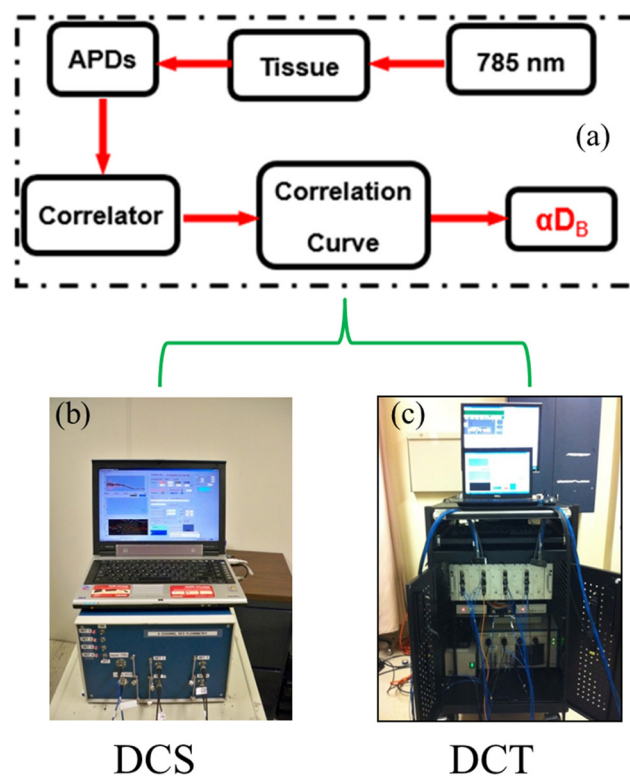
Figure 2. The schematic diagram (a) and instrument photos of typical DCS (b) and DCT (c) systems.
