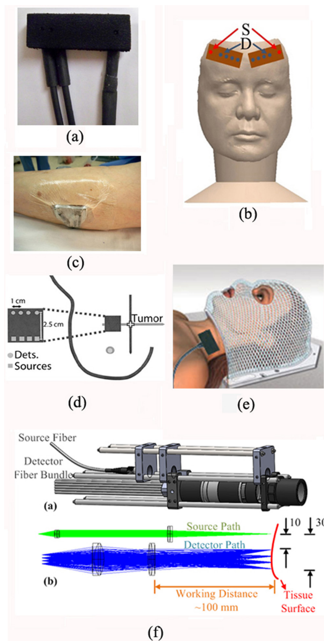
Figure 3. A variety of optical probes for DCS/DCT measurements. (a) A typical DCS probe consisting of source and detector fibers; (b) two DCS probes taped on both sides of a frontal head for cerebral blood flow measurements; (c) a DCS probe taped on top of the calf muscle; (d) a hand-held DCS probe scanning over a breast tumor; (e) a DCS probe placed on top of the head/neck tumor; (f) a noncontact DCS probe with lens system focusing the source and detectors on the surface of tissue. Some of the figures are reproduced from the subfigures in Durduran et al (2005) and Huang et al (2015c)
