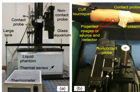
Fig. 2 Experimental setup for concurrent flow measurements using contact and noncontact probes in a liquid phantom solution (a) and a forearm muscle (b).
