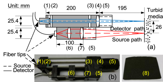
Fig. 1 Schematic (a) and photograph (b) of the noncontact probe including (1) collimator, (2) longpass optical filter, (3) aperture, (4) 200 mm FL lens, (5) protection tube, (6) 50 mm FL lens, (7) 250 mm FL lens and (8) crepe black weave.
