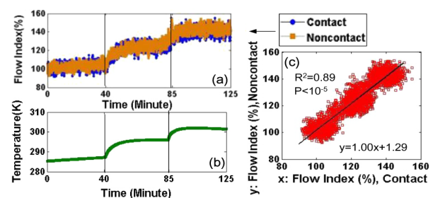
Fig. 3 Relative flow changes (a) measured by the contact and noncontact probes during temperature variations (b) are highly correlated (c). The vertical lines in (a) and (b) represent the time points to fill hot water (twice) into the large tank [see Fig. 2(a)].
